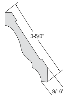
CROWN MOULDING
