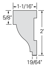
RAKE MOULDING #5287P16
