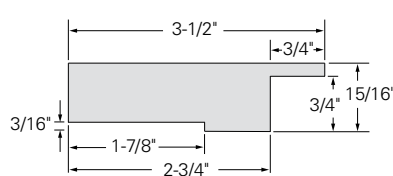
KLEER KONCEAL® TRIMBOARD WITH NAILING FLANGE CUTOUT
