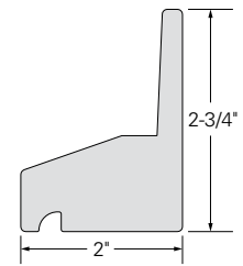
WATER TABLE #5170C18
