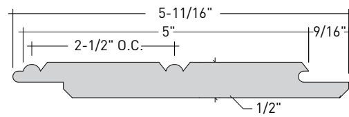
6" KLEERLOK® BEADED BOARD
